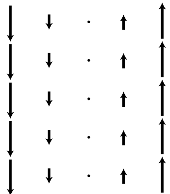
e / The field x\hat{y} .
